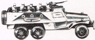
11 BTR 152 C 6-Rad-Schützenpanzer 1,50 DM (ohne Fig.) BTR 152 C U.R.S.S., Vehicule de transport d'infanterie (sans figures) BTR 152 C armoured personnel carrier (without figures)
